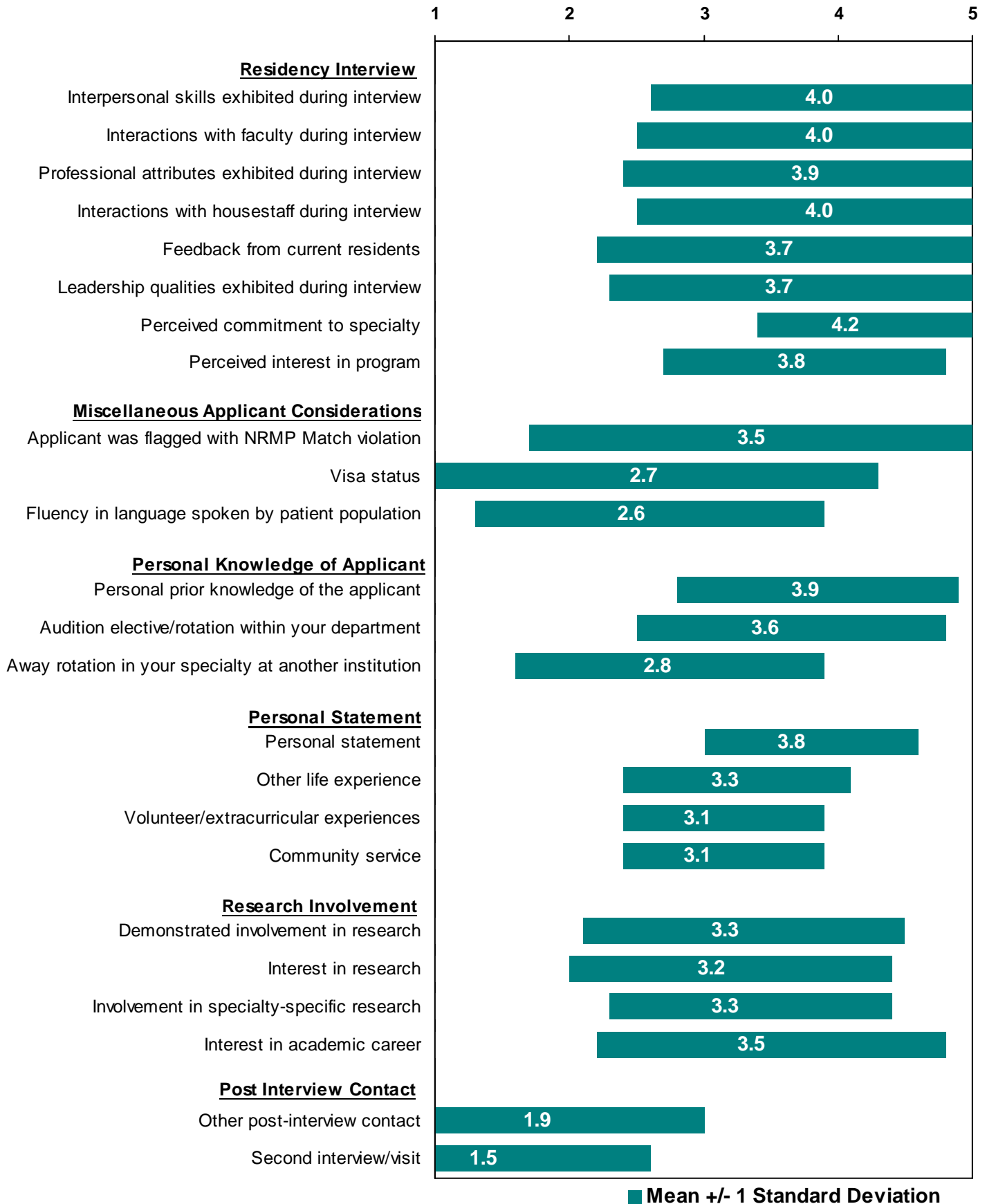
Figure DM-2 (continued)
